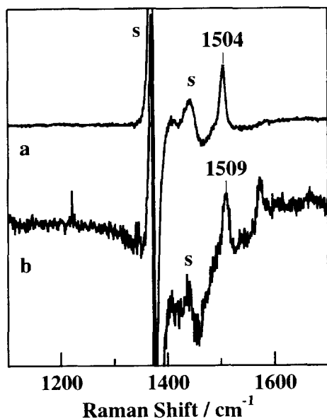
Fig. 8. Resonance Raman spectra of the one-electron-oxidized species of 2 and [\text{ZnCl}(\text{tbuL})] ; a, 2 ; b, [\text{ZnCl}(\text{tbuL})] . Solvent peaks are subtracted and s denote the residues from the solvent peaks. The concentration of the sample was 0.5 mM.
